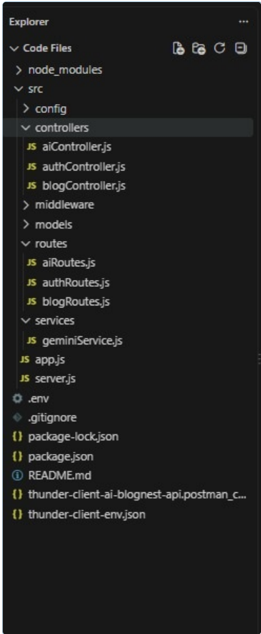
Fig. - Actual Server/ project folder structure (VS Code Explorer).
